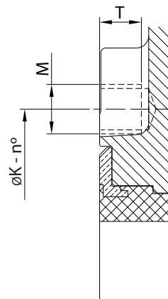
DN 10"
