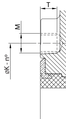
DN 300
